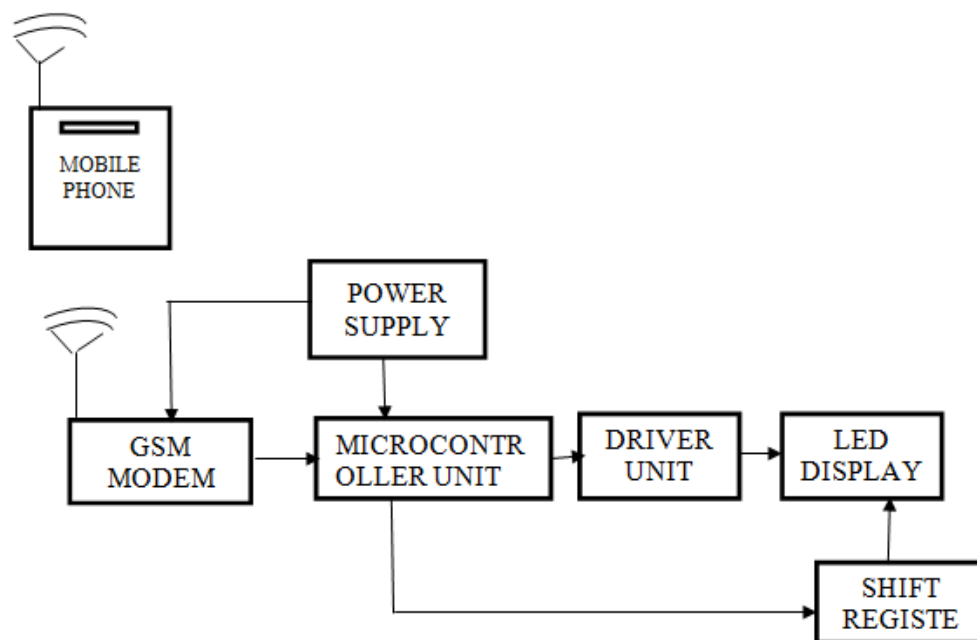
Figure1: Block Diagram of Microcontroller Based Electronic Billboard
