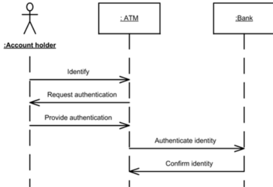
Gambar 1.4. Sequence diagram.
