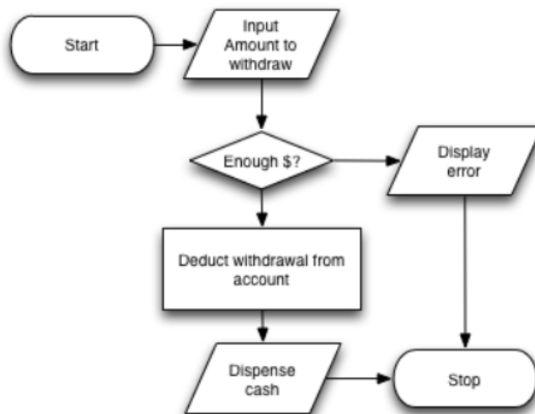
Gambar 1.2. Flowchart .
