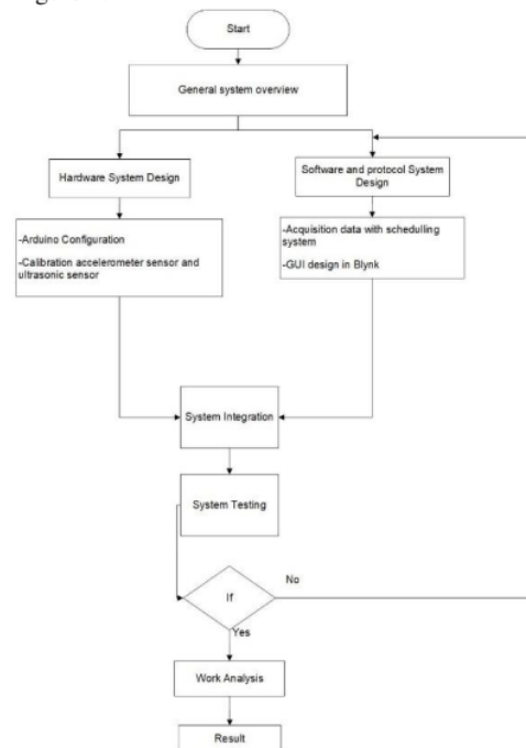
Figure 1. Flowchart System
