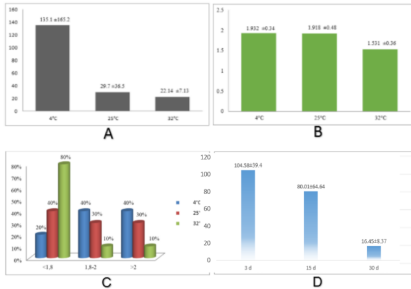
Figure 1. Effect of temperature and storage duration on DNA quality A. DNA Concentration treated by temperature (ng/μl) ( Kruskal Wallis <0.05). B. Purity of DNA (A 260/280) (one way anova, p>0.05 ). C. Percentage of Purity level of DNA influenced by temperature, D. DNA Concentration treated by storage duration ( Kruskal Wallis , p<0.05 )
