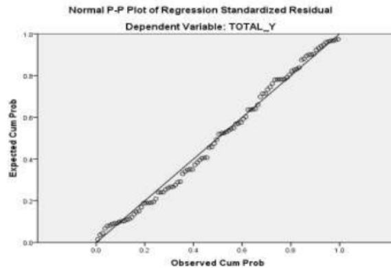
Gambar 2. Normality Test
