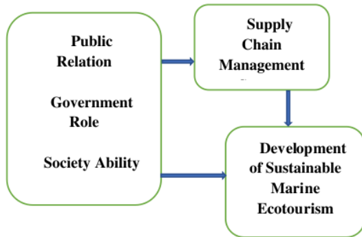
Figure 1. Theoretical framework
