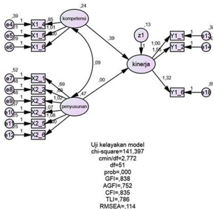
Figure 2: Research model after invalid indicator being eliminated
