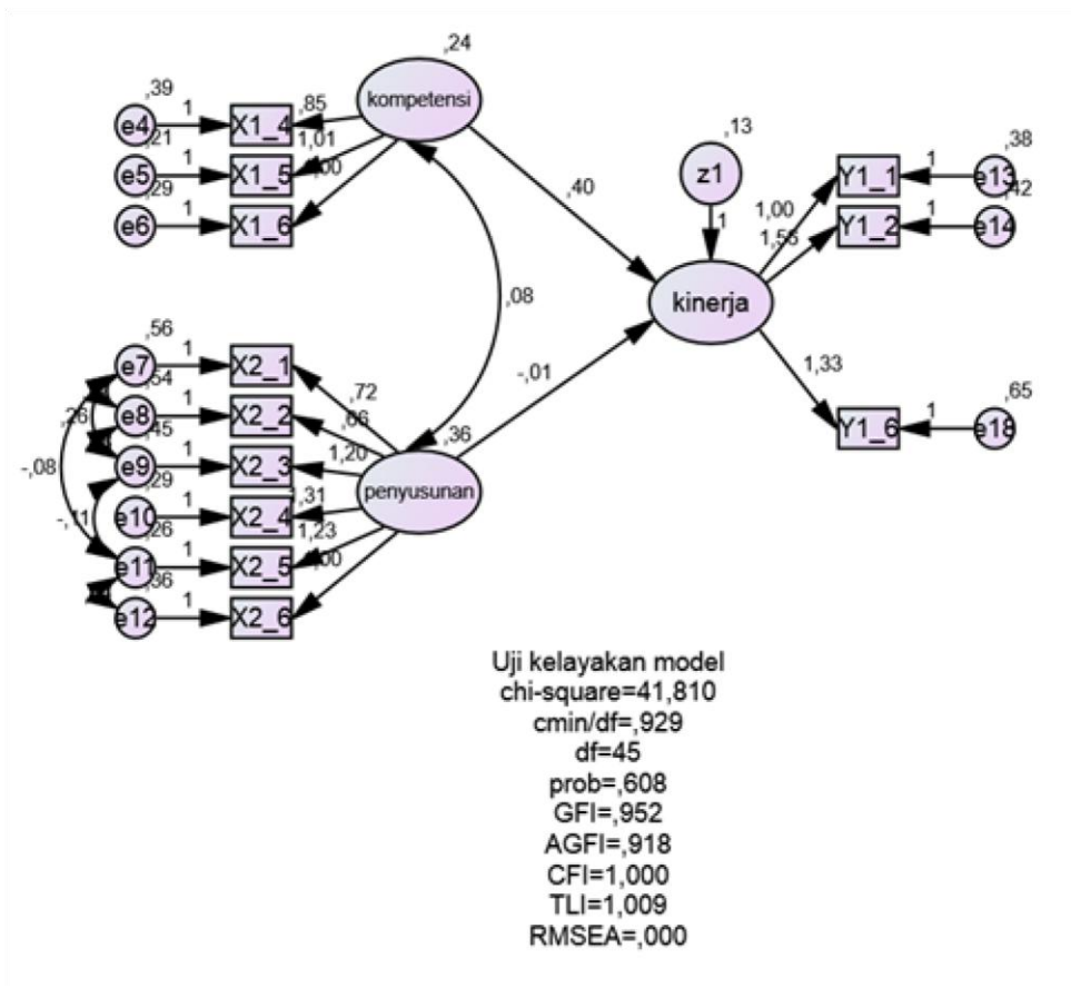
Figure 4: Output SEM model trajectory diagram modification
