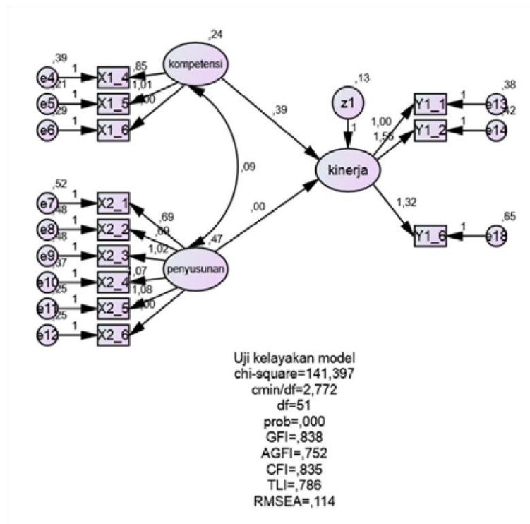
Figure 3 Diagram Output of Early SEM Trajectory Model
