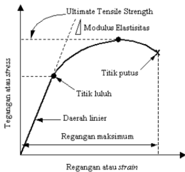
Gambar 1. Diagram Tegangan-Regangan
