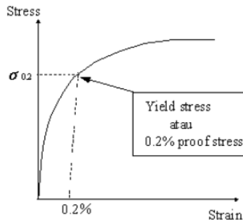
Gambar 2. Penentuan tegangan luluh ( yield stress )
