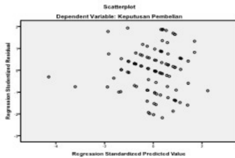
Figure 1. Uji Heteroskedasitas
