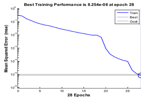
Figure 4. Performance performance results of the identification of Backpropagation (20-15-15-1)
