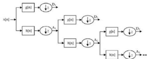
Fig.1: Sub-decomposition of Discrete Wavelet Transforms
