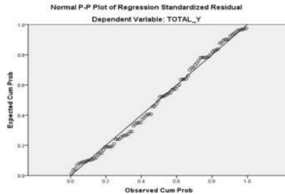
Gambar 2. Normality Test
