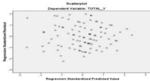
Gambar 3. Heterocedasticity test
