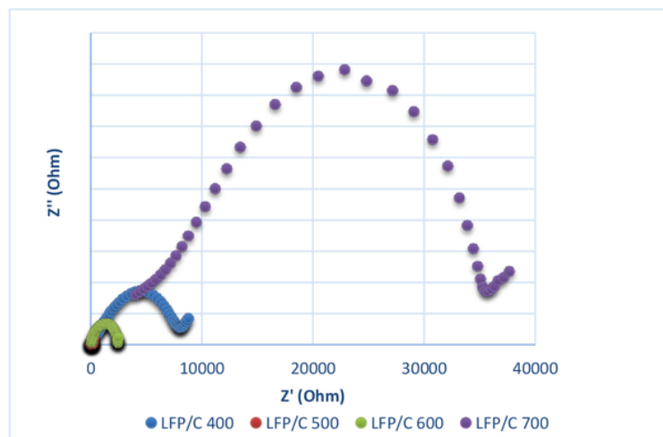
Figure 2. Total impedance value curve of LFP/C composite material at various calcination temperature (400 °C, 500°C, 600°C and 700°C)
