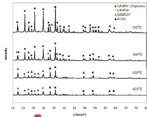
Figure 1. The XRD pattern of LFP/C composites by solid-state reaction methods at 400°C, 500°C, 600°C, and 700°C
