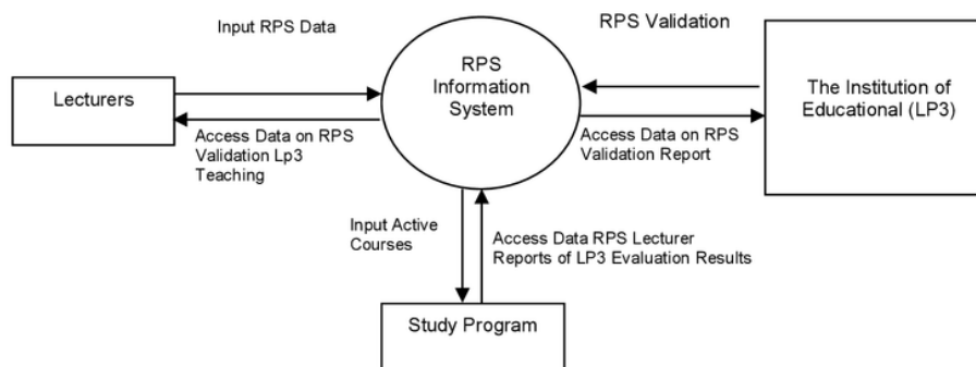
Figure 2. DFD Level 0 of Teaching Plan Information System
