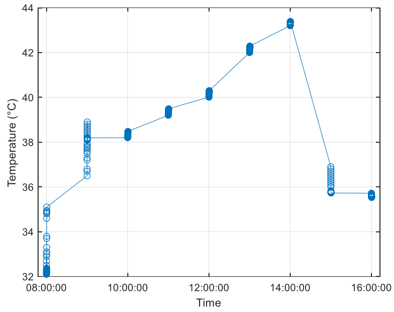
Figure 9. Heat intensity of solar panels
