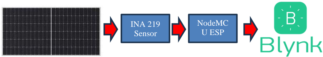
Figure 2. NodeMCU ESP 8266 System with Solar Panel
