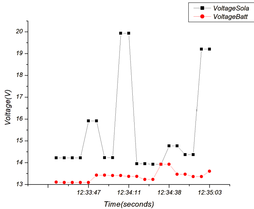
Figure 6. Compariso between Voltage Solar Panels and Battery
