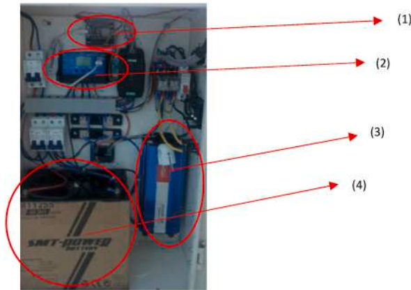
Fig. 5. Solar panel control hardware.
