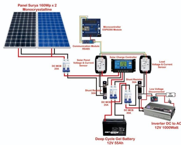
Figure 3. Dual Axis Solar Tracker Instrumentation System Design with LDR and ESP 8266
