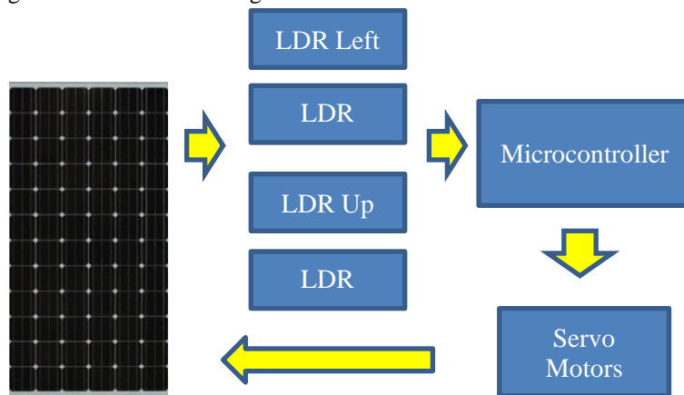
Figure 1. Block Diagram of Dual Axis Solar Tracker Movement Instrumentation System
