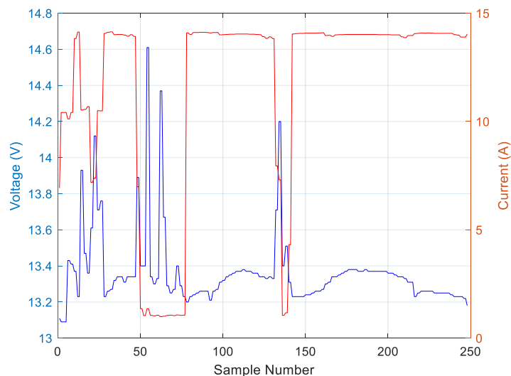
Figure 6. Graphic of Solar Panel Voltage and Current Measurements
