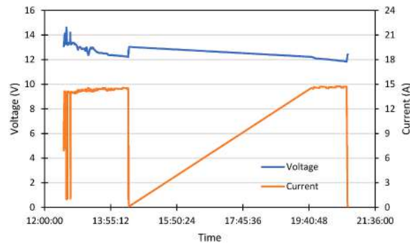
Fig. 8. Result of battery instrumentation.
