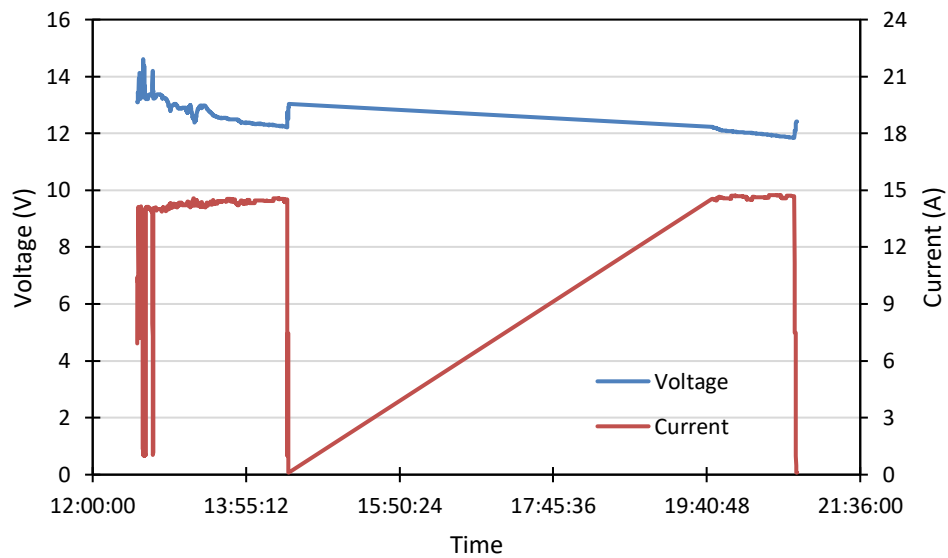
Figure 8. Result of Battery Instrumentation
