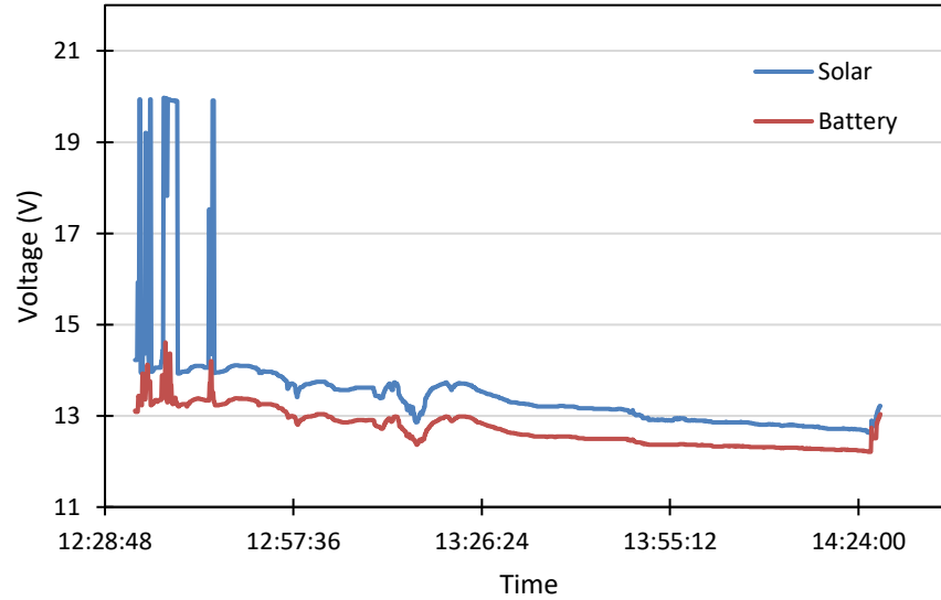
Figure 7. Comparison between voltage solar panels and battery
