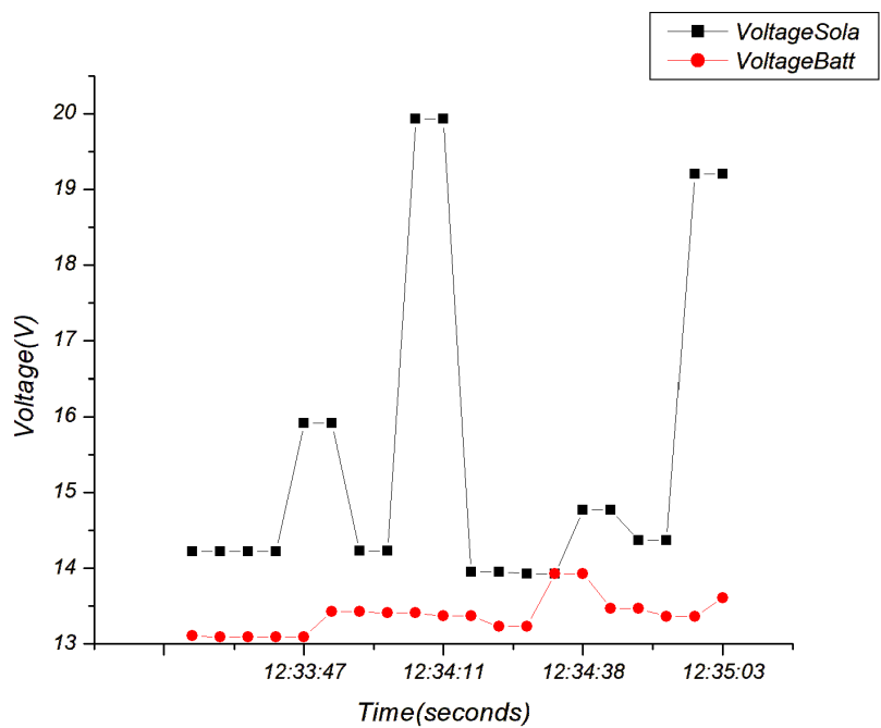
Figure 6. Comparison between Voltage Solar Panels and Battery
