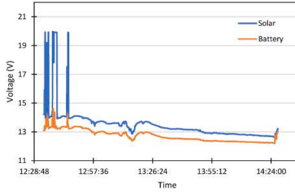
Fig. 7. Comparison between voltage solar panels and battery.
