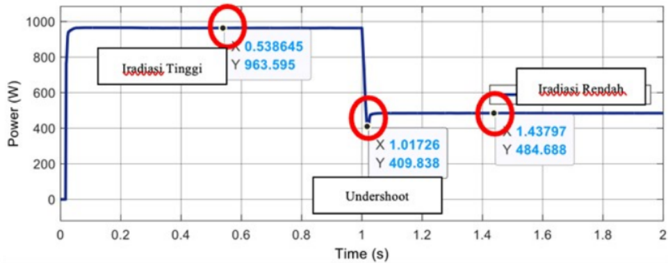
Figure 6. Hasil daya PV tipe filter lowpass
