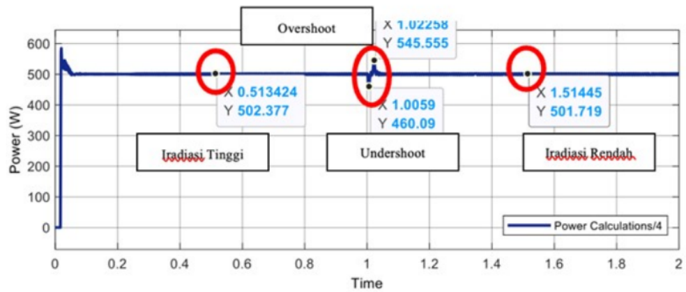
Figure 7. Hasil daya beban tipe filter lowpass
