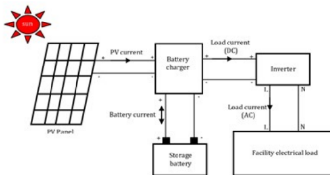
Figure 1. Konsep sistem panel surya off-grid [1]
