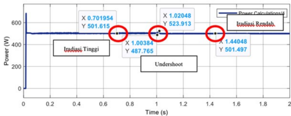
Figure 10. Hasil daya beban tipe filter highpass
