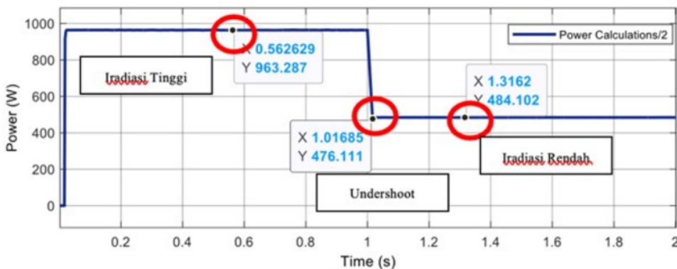
Figure 9. Hasil daya PV tipe filter highpass
