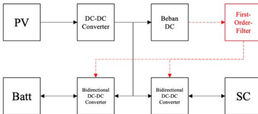
Figure 5. Blok diagram keseluruhan penelitian
