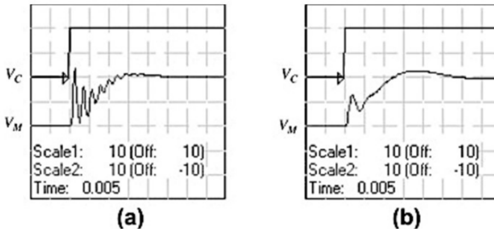
Figure 4. Hasil output first-order filter (a) sebelum (b) sesudah [15]
