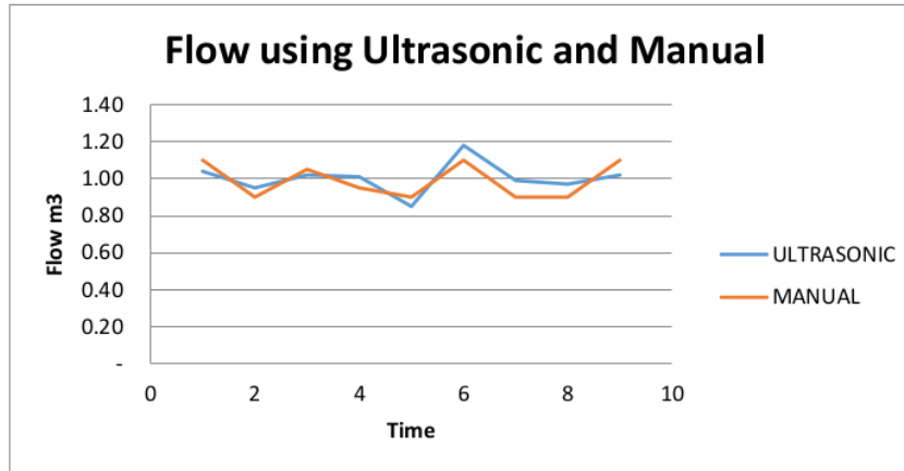
Fig. 10. Flow using Ultrasonic and Manual
