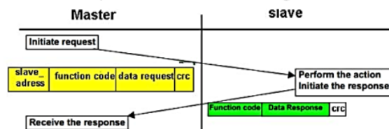
Fig. 9. Modbus Transaction Error
