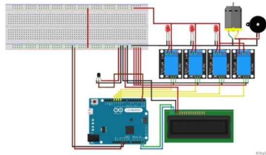
Gambar 1. Wiring System
