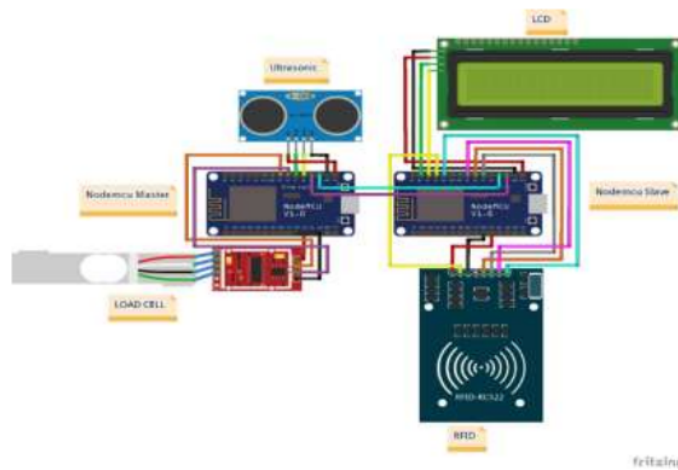
Figure 1. Wiring Design
