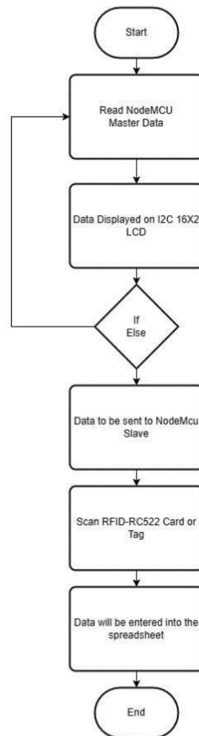
Figure 3. Slave Flowchart Program
