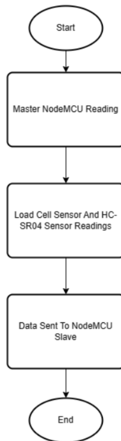
Figure 2. Master Flowchart Program
