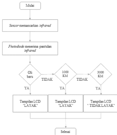
Gambar II.2 Flowchart alat
