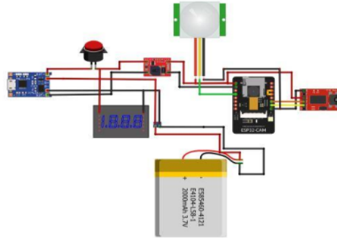
Figure 3. Tool Connection
