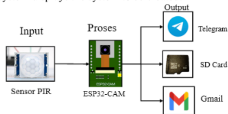
Figure 2. Block Circuit Diagram
