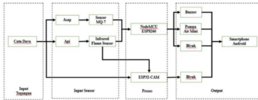
Gambar 9. Blok Diagram
