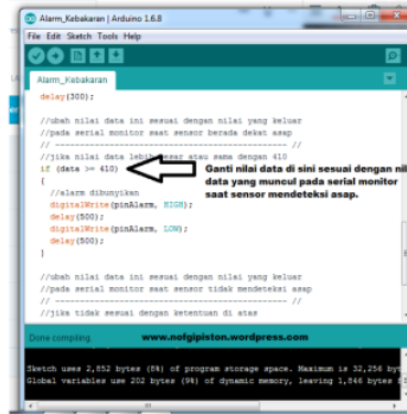
Gambar 12. Program Arduino IDE
