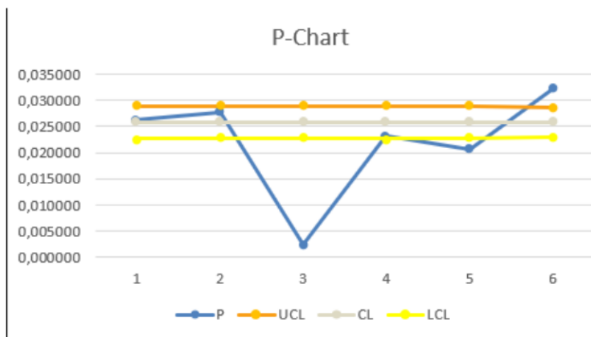
Figure 6. Diagram P chart
