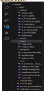
Gambar 5. File-file View
