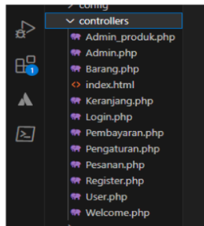
Gambar 4. File-file Controller
