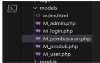
Gambar 3. File-file Model
