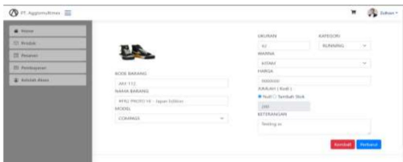
Gambar 18 Edit Barang
