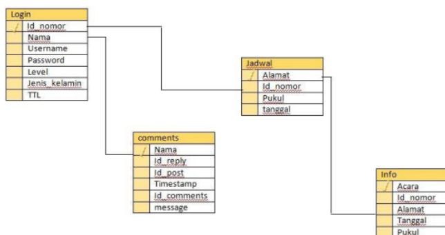
Gambar 2. Database
