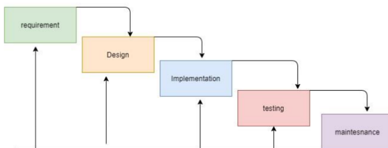
Gambar 1. Metode Waterfall
