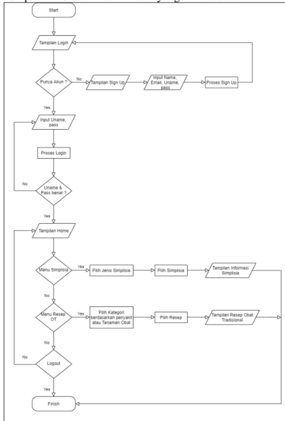
Gambar 2 Flowchart system
