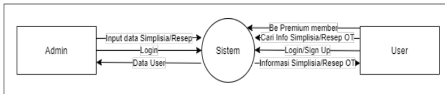
Gambar 3 DFD Level 0
