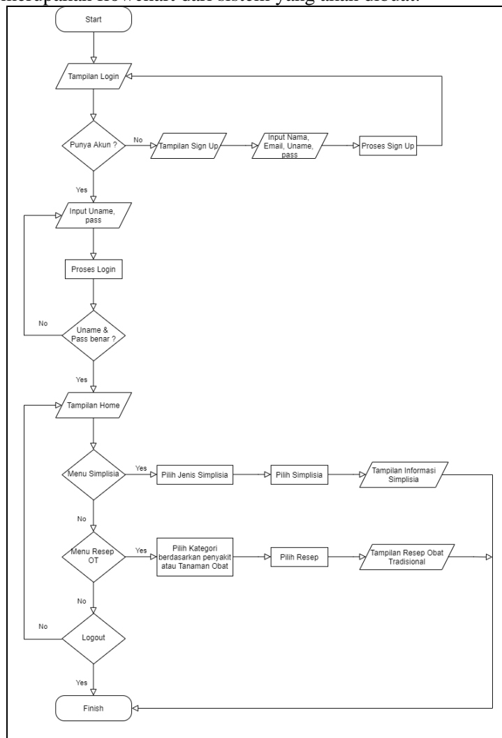
Gambar 2 Flowchart system
