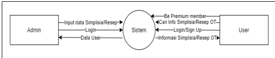
Gambar 3 DFD Level 0
