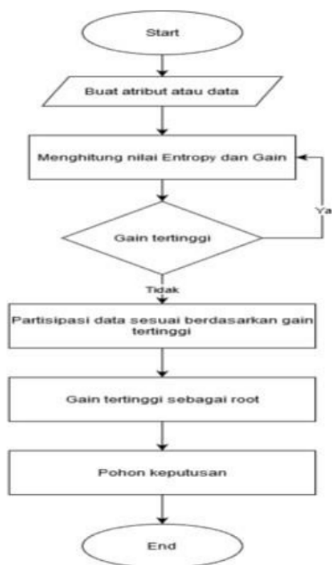
Figure 1. Alur algoritma C4.5
