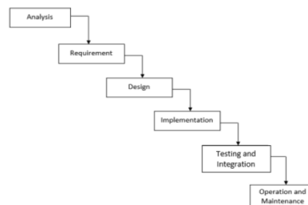
Gambar 1. Metode Waterfall
