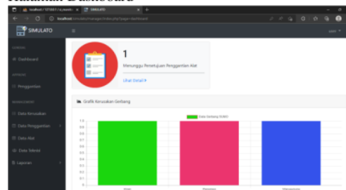
Gambar 10. Halaman Dashboard
