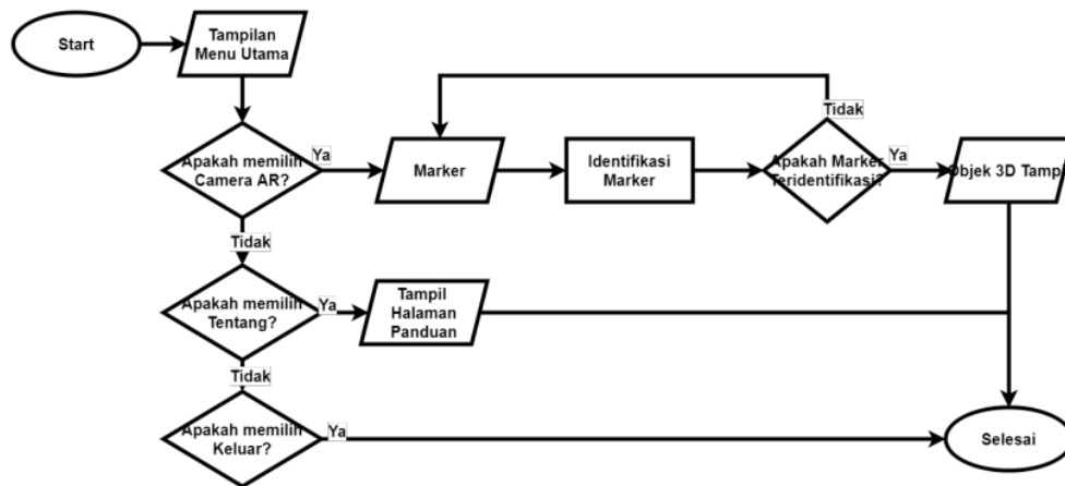
Gambar 1. Flowchart
