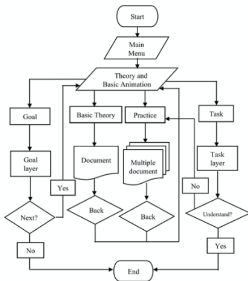
Fig. 1. Multimedia flowchart
