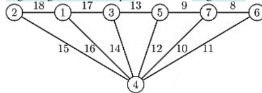
Figure 4. Labeling of graph fan F_6 .
