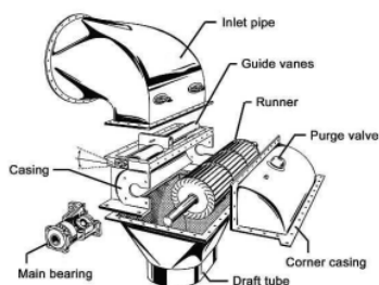
Gambar 1. Turbin Cross flow
