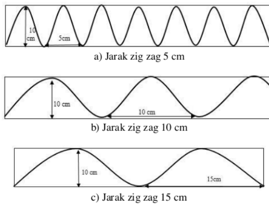
Gambar 2. Variasi jarak zig-zag pengisi cooling tower
