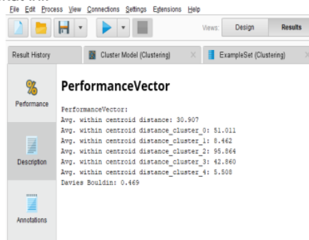
Gambar 5. Centroid Distance K-Means
