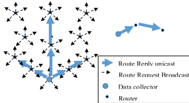
Gambar 6 Many to one route [4] [10]
