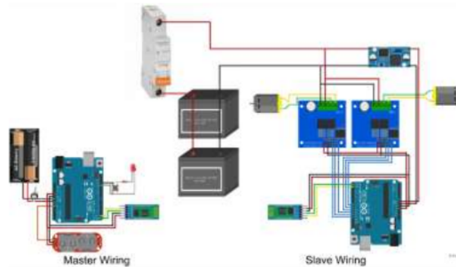
Fig. 1 Wiring Design
