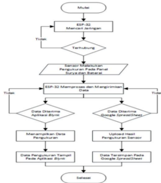
Gambar 7. Flowchart
