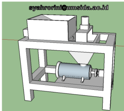
Figure 3. Hardware Design View Left
