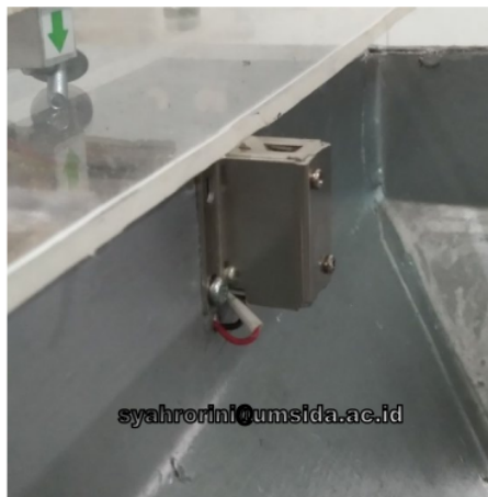
Figure 11. Solenoid Doorlock Condition When Load 1 kg
