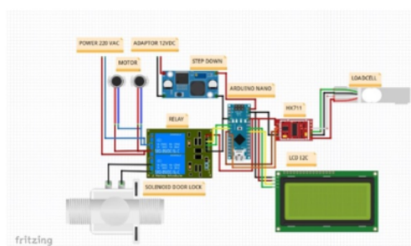
Figure 2. Organic Waste Crushing Machine Automatic Wiring Design
