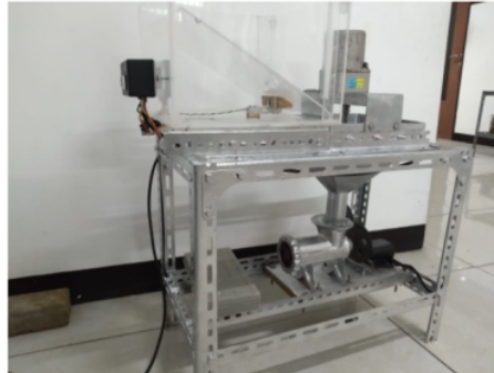
Figure 6. Automation of Organic Waste Shredder
