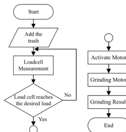
Figure 1. Flowchart System
