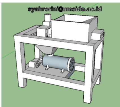
Figure 4. Right View Design
