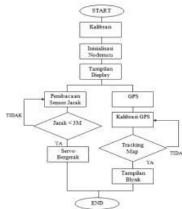
Gambar 1. Flowchart Sistem
