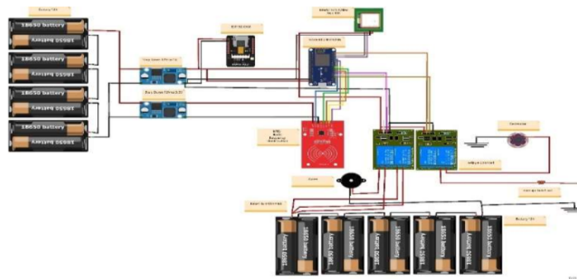
Gambar 9. Wiring diagram
