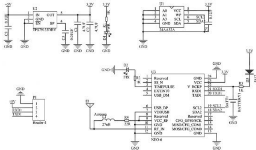
Gambar 1. Diagram Wiring Modul Gps U-Blox 6 M
