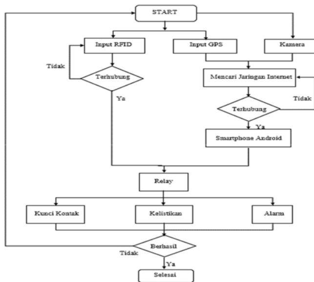
Gambar 8. Flowchart system
