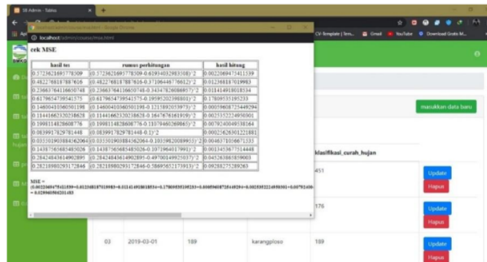
Figure 2. Mean Squared Error (MSE) calculation.
