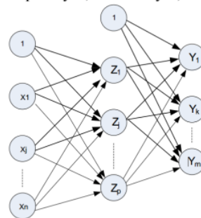
Figure 1. Backpropagation architecture.
