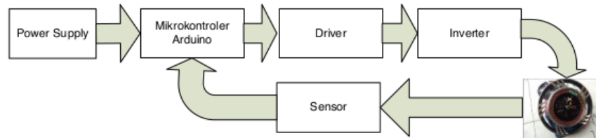
Gambar 5. Hardware Monitoring Perubahan Tegangan
