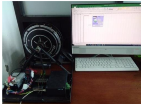
Gambar 7. Hardware Monitoring Perubahan Tegangan Motor BLDC
