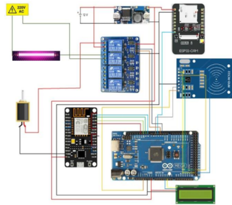
Fig 4. Wiring design
