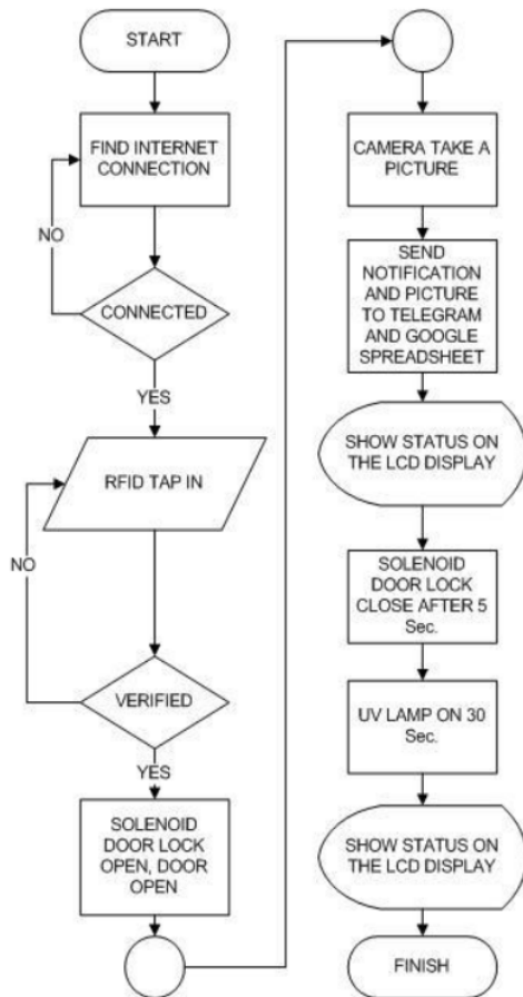
Fig 3. Flowchart program
