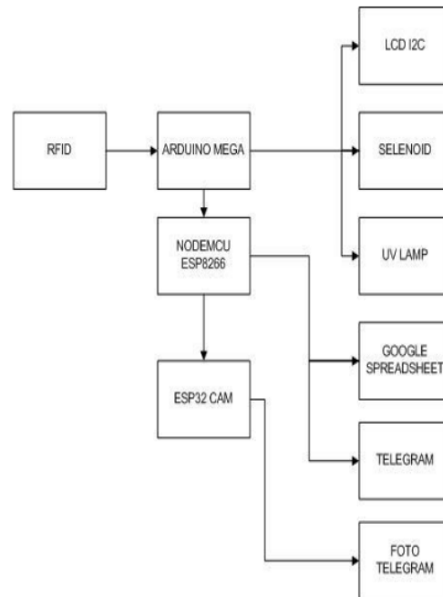
Fig 2. Tool Block Diagram
